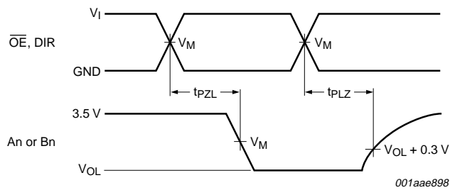
Fig 9. 3-state output enable time to LOW-level and output disable time from LOW-level
