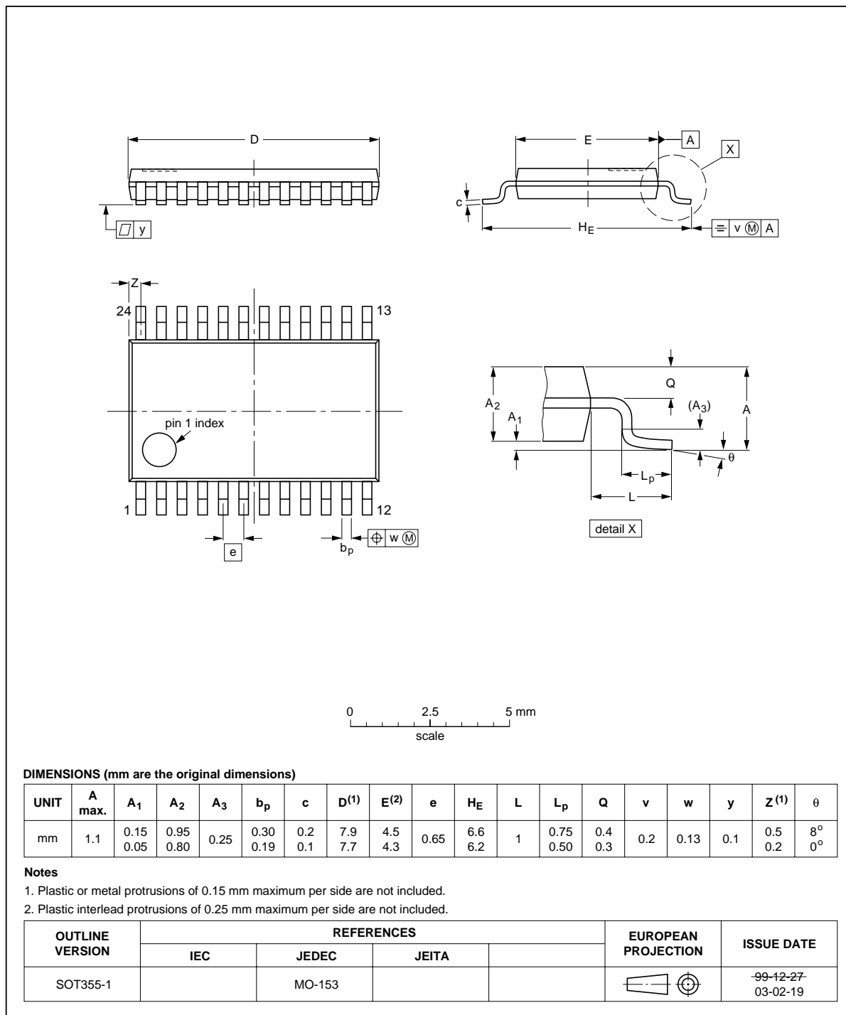
Fig 14. Package outline SOT355-1 (TSSOP24)
