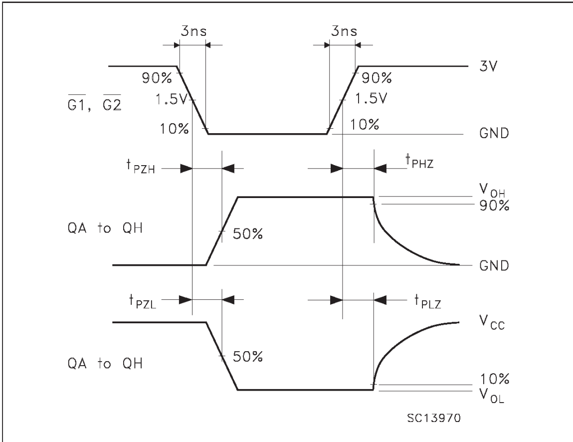
WAVEFORM 4: PROPAGATION DELAYS ( f=1\text{MHz} ; 50% duty cycle)
