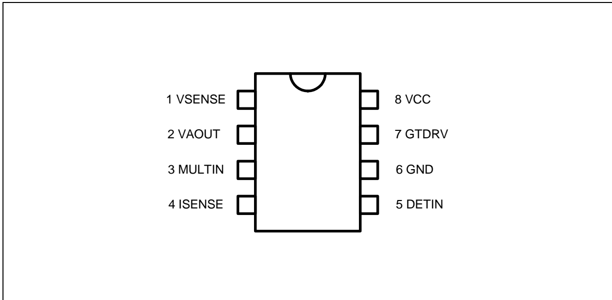
Figure 2 Pin Configuration of TDA4863
