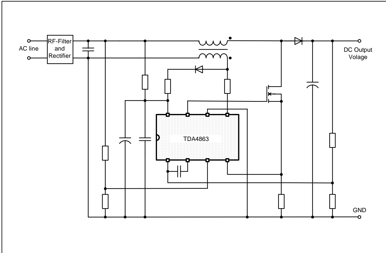
Figure 1 Typical application
