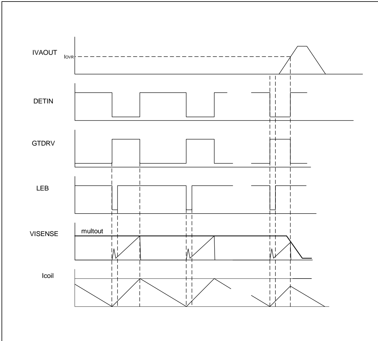
Figure 4 Typical signals
