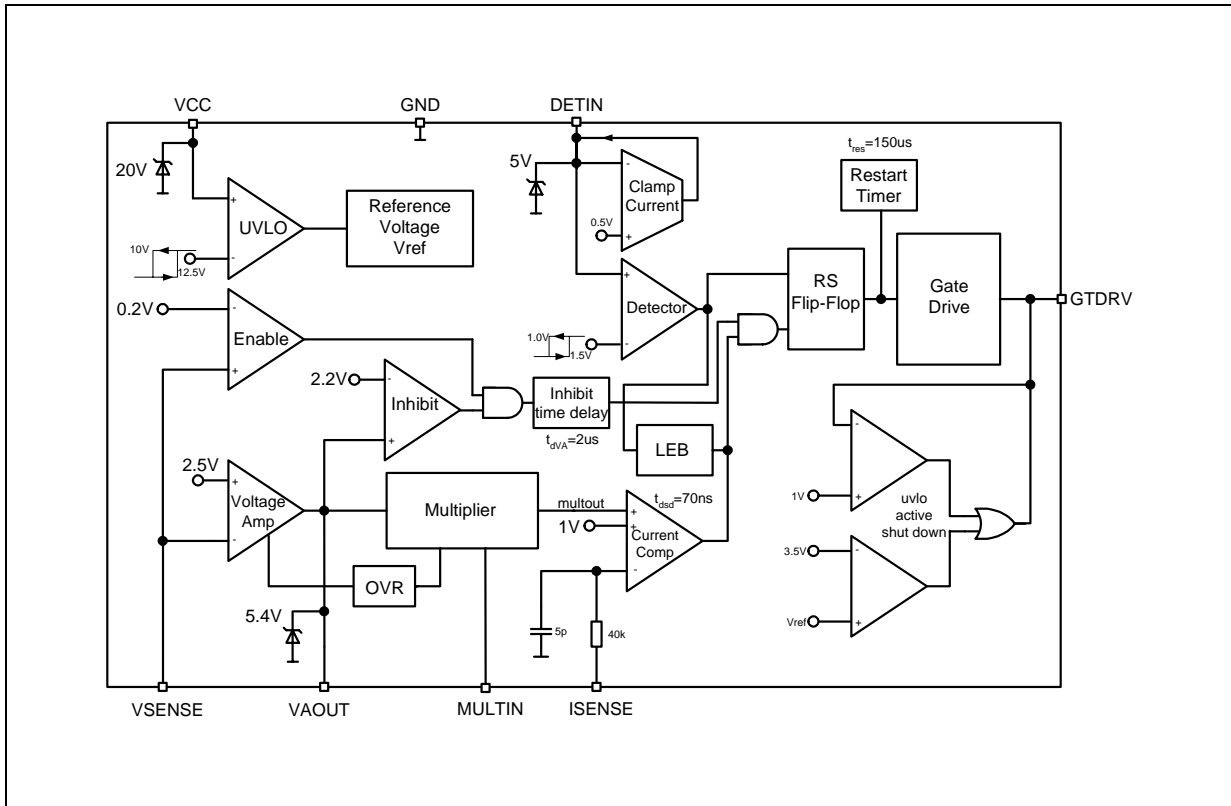
Figure 3 Internal Block Diagram
