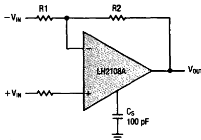
Alternate Frequency Compensation
