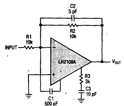
Feedforward Compensation
