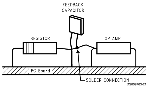
FIGURE 10. Air Wiring
