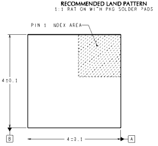
8-Lead LLP Order Number LM2940LD-5.0, LM2940LD-8.0, LM2940LD-9.0, LM2940LD-10, LM2940LD-12 or LM2940LD-15 NS Package Number LDC08A
