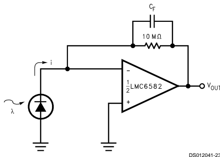
FIGURE 17. Photodiode Amplifier
