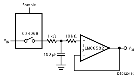
FIGURE 22. Sample-and-Hold Application
