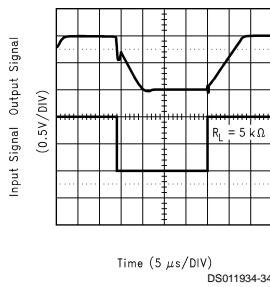
Non-Inverting Large Signal Pulse Response
