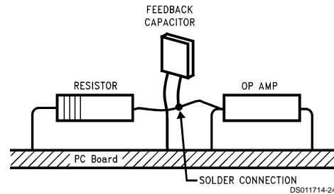
FIGURE 11. Air Wiring
