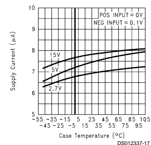
Supply Current vs Temperature while Sinking
