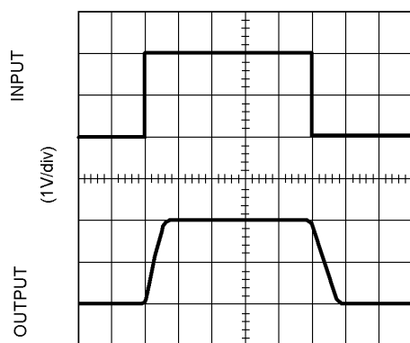
Non-Inverting Large Signal Pulse Response, V_S = 2.7V
