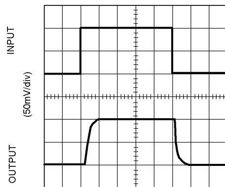
Non-Inverting Small Signal Pulse Response, V_S = 2.7V
