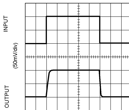
Non-Inverting Small Signal Pulse Response, V_S = 5V
