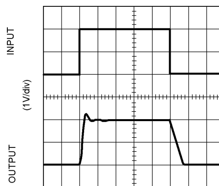
Non-Inverting Large Signal Pulse Response, V_S = 5V
