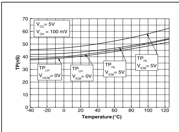
Figure 23. Propagation delay vs. temperature V_{CC}=5V , overdrive=100mV
