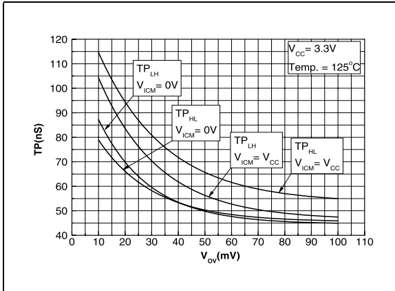
Figure 19. Propagation delay vs. overdrive V_{CC}=3.3V
