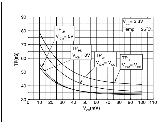
Figure 17. Propagation delay vs. overdrive V_{CC}=3.3V
