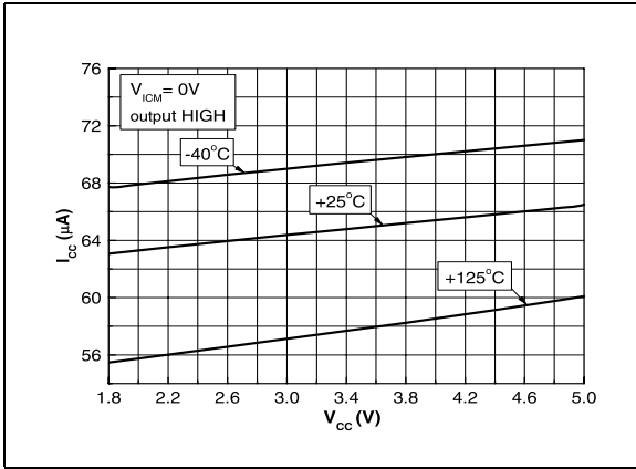
Figure 1. Current consumption vs. power supply voltage
