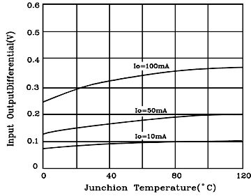
Dropout Voltage
