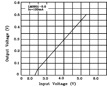
Low Voltage Behavior
