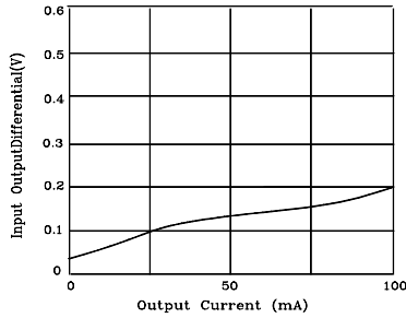
Dropout Voltage
