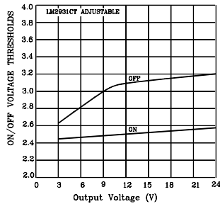
On/Off Threshold
