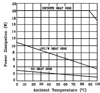
Maximum Power Dissipation (TO-220)
