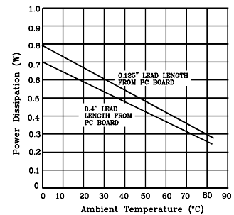
Maximum Power Dissipation (TO-92)
