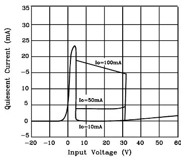
Quiescent Current
