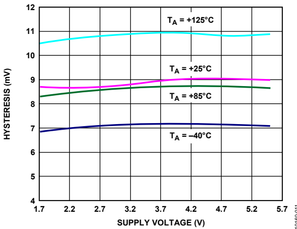
Figure 11. Hysteresis vs. Supply Voltage
