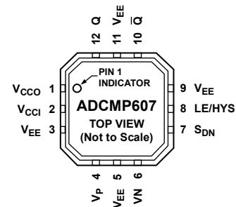
Figure 2.LFCSP Pin Configuration
