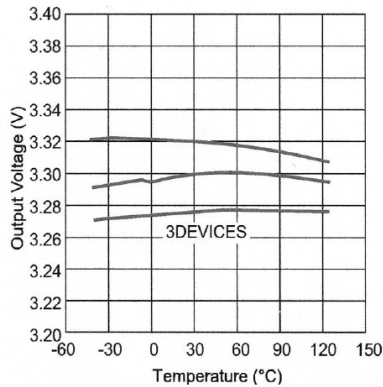
LM29150-3.3 Output Voltage vs. Temperature
