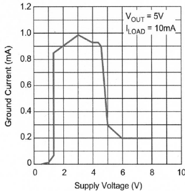
LM29150 Ground Current vs. Supply Voltage
