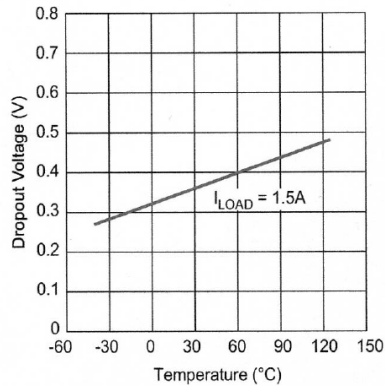
LM29150 Dropout Voltage vs. Temperature
