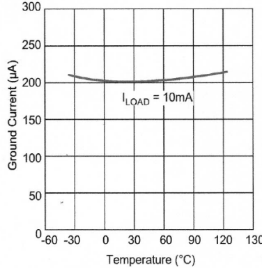
LM29150 Ground Current vs. Temperature
