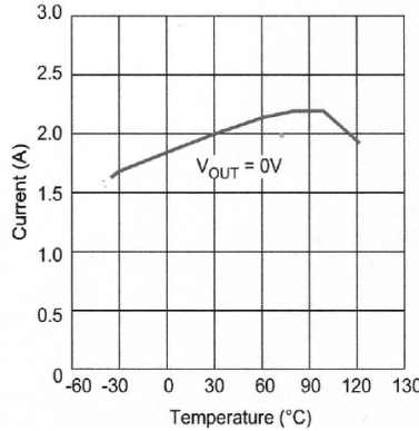
LM29150-3.3 Short Circuit Current vs. Temperature
