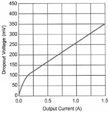
LM29150 Dropout Voltage vs. Output Current
