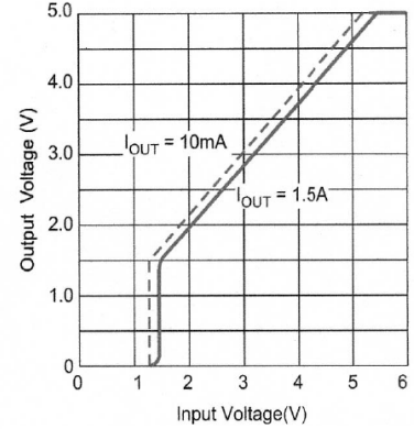
LM29150-5.0 Dropout Characteristics
