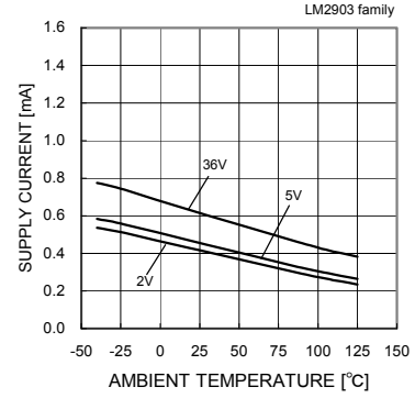
Fig. 43 Supply Current - Ambient Temperature
