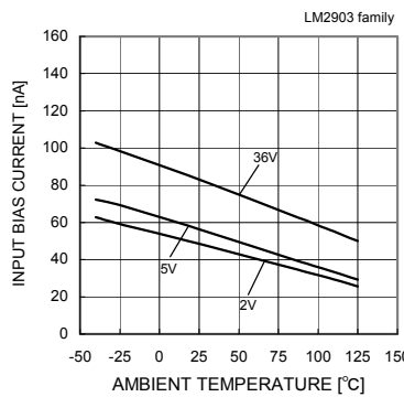
Fig. 51 Input Bias Current - Ambient Temperature
