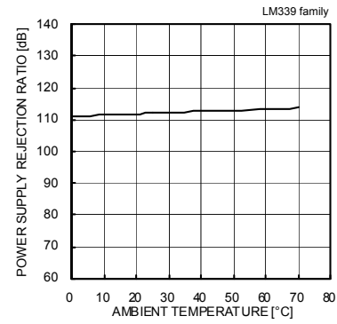
Fig. 38 Power Supply Rejection Ratio – Ambient Temperature
