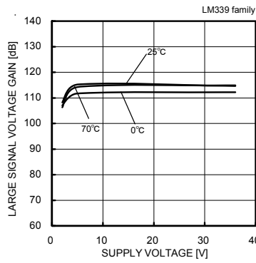
Fig. 34 Large Signal Voltage Gain – Supply Voltage
