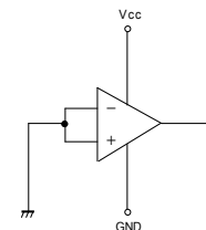
Fig.92 Disable circuit example
