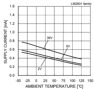
Fig. 66 Supply Current - Ambient Temperature
