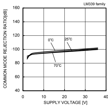
Fig. 36 Common Mode Rejection Ratio – Supply Voltage
