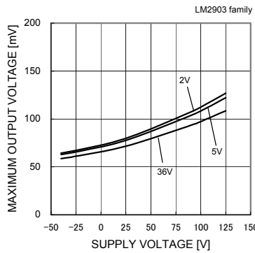
Fig. 45 Output Saturation Voltage - Ambient Temperature (IOL=4[mA])
