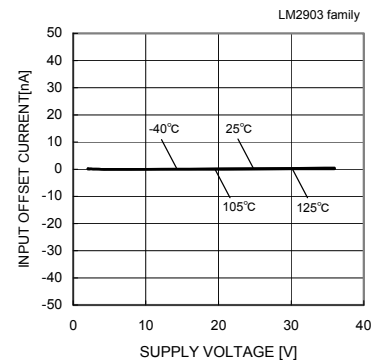
Fig. 52 Input Offset Current - Supply Voltage
