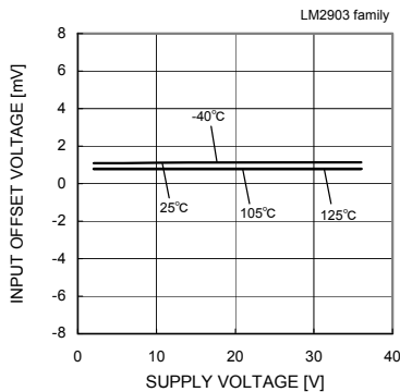
Fig. 48 Input Offset Voltage - Supply Voltage
