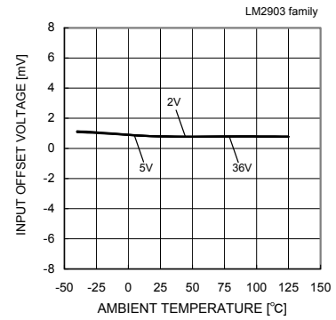
Fig. 49 Input Offset Voltage - Ambient Temperature
