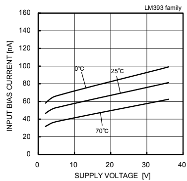
Fig. 10 Input Bias Current - Supply Voltage
