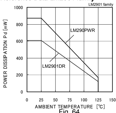
Fig. 64 Derating Curve
