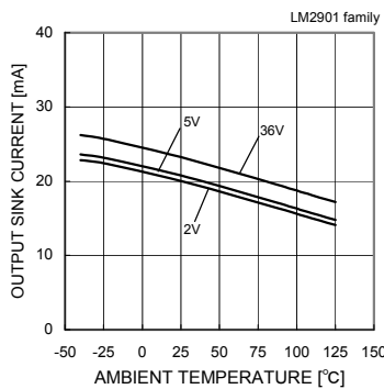
Fig. 70 Output Sink Current - Ambient Temperature (VOUT=1.5[V])
