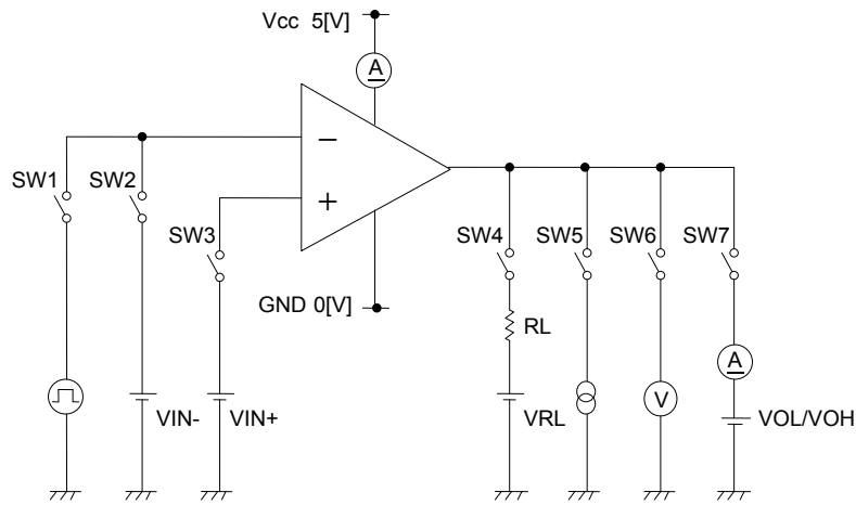
Fig.89 Measurement Circuit2 (each channel)
