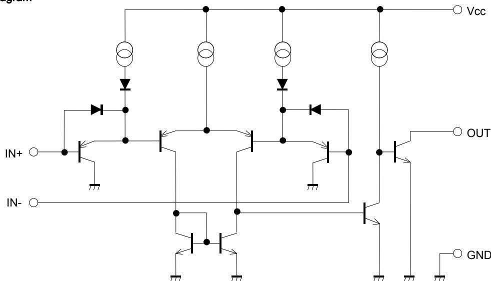
Fig.87 Circuit Diagram (each Comparator)
