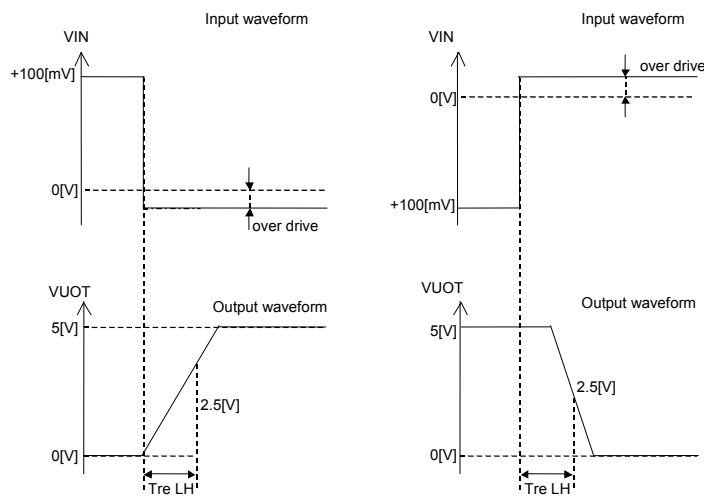
Fig.90 Response Time
