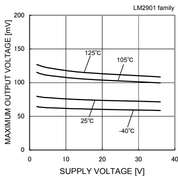
Fig. 67 Output Saturation Voltage - Supply Voltage (IOL=4[mA])
