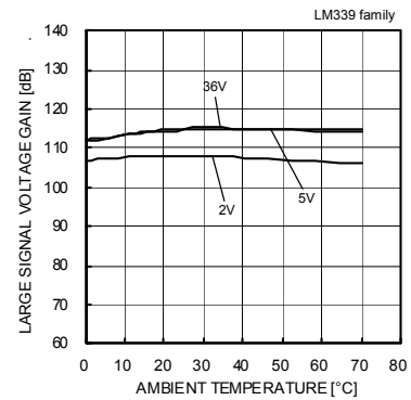
Fig. 35 Large Signal Voltage Gain – Ambient Temperature
