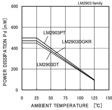
Fig. 41 Derating Curve
