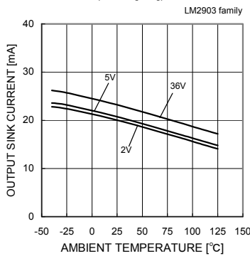
Fig. 47 Output Sink Current - Ambient Temperature (VOUT=1.5[V])
