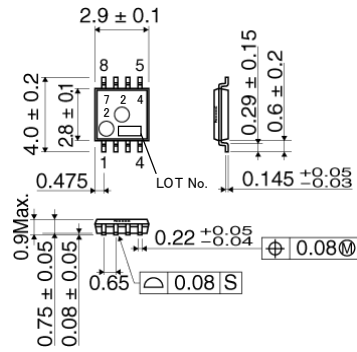
BU7242FVM (MSOP8) (Unit : [mm])
