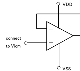
Fig.1 The example of disabled circuit
