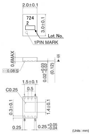
BU7242NUX (VSON008X2030) (Unit : [mm])
