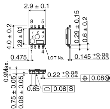
BU7242SFVM (MSOP8) (Unit : [mm])
