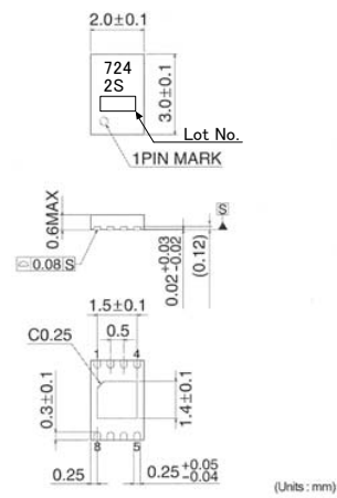
BU7242SNUX (VSON008X2030) (Unit : [mm])
