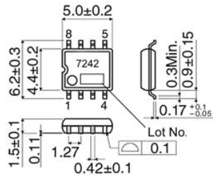
BU7242F (SOP8) (Unit : [mm])
