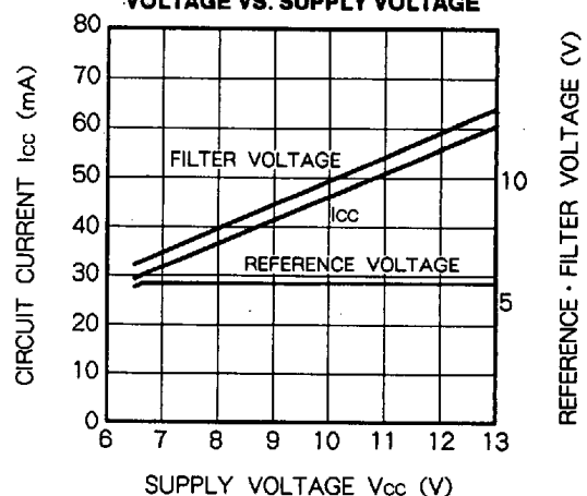
CIRCUIT CURRENT, REFERENCE-FILTER VOLTAGE VS. SUPPLY VOLTAGE
