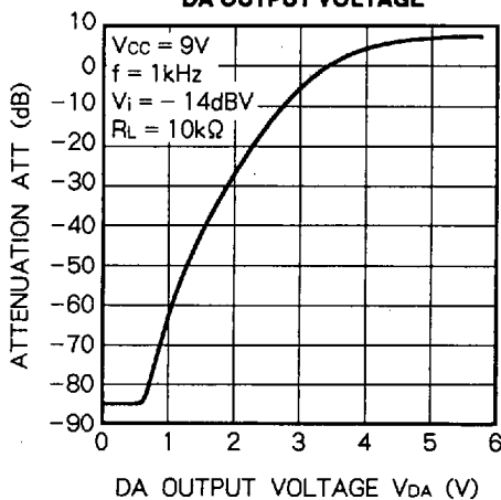
VCA ATTENUATION VS. DA OUTPUT VOLTAGE
