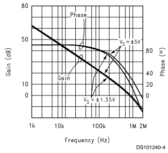
Gain/Phase vs. Frequency R_L = \text{open}
