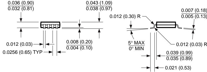
8-Pin MSOP (MM)
