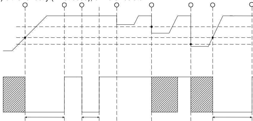
Figure 8 – Power-On / Brown-out Reset Conditions
