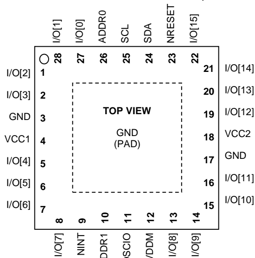
Figure 3 – SX1509QB QFN-UT-28 Pinout
