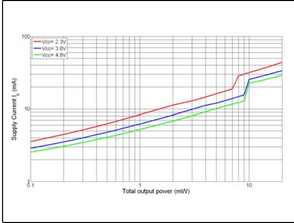
Figure 8. Current consumption vs. total output power, R_L = 32 \Omega
