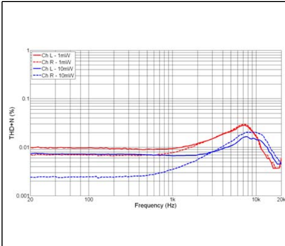
Figure 46. THD+N vs. frequency, R_L = 32 \Omega , out-of-phase, V_{CC} = 4.8 V
