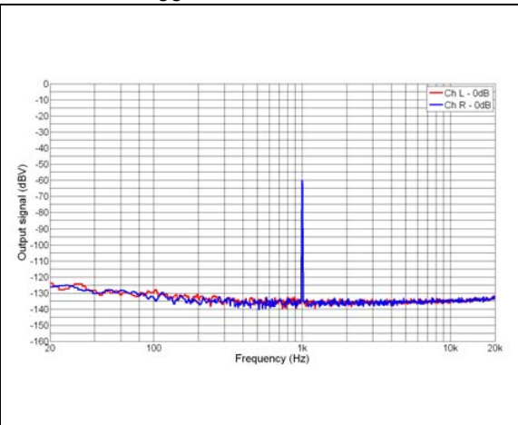
Figure 55. Output signal spectrum ( V_{CC} = 3.6 V , load = 32 \Omega )
