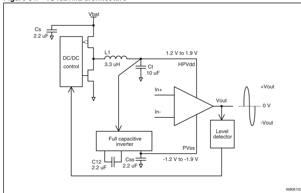
Figure 64. TS4621ML architecture
