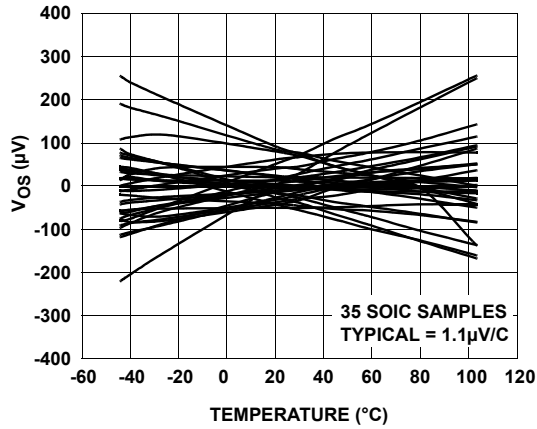
FIGURE 13. EL8178 SOIC V_{OS} vs TEMPERATURE ( V_S = 5V )
