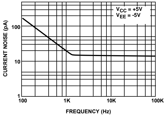
FIGURE 13. CURRENT NOISE
