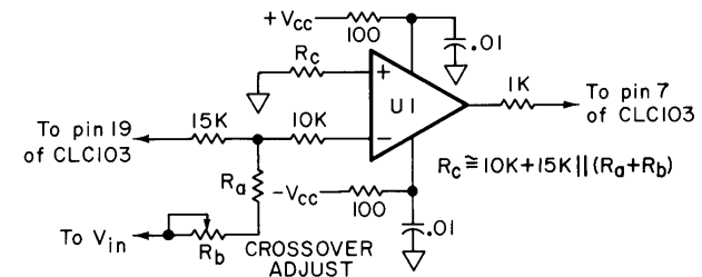
Figure 4: inverting gain composite amplifier to be used with figure 2 circuit
