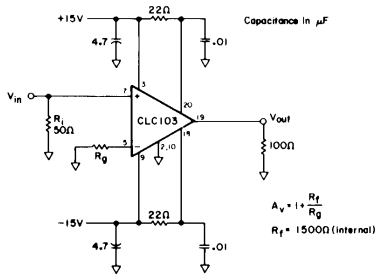
Figure 1: recommended non-inverting gain circuit
