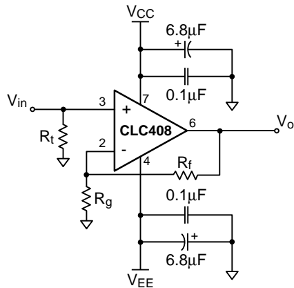
Figure 1: Non-Inverting Gain
