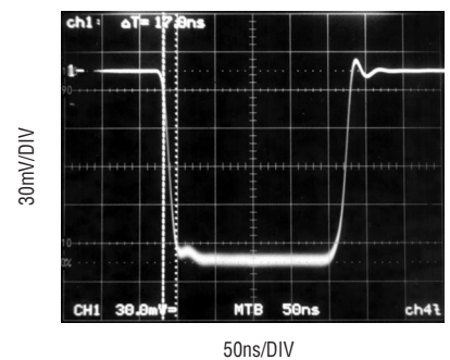
Photodiode Amplifier Time Domain Response
