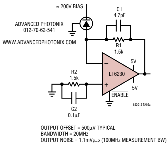
Low Power Avalanche Photodiode Transimpedance Amplifier I_{\text{S}} = 3.3\text{mA}
