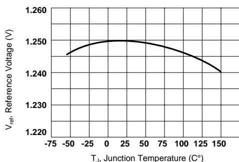
TEMPERATURE STABILITY
