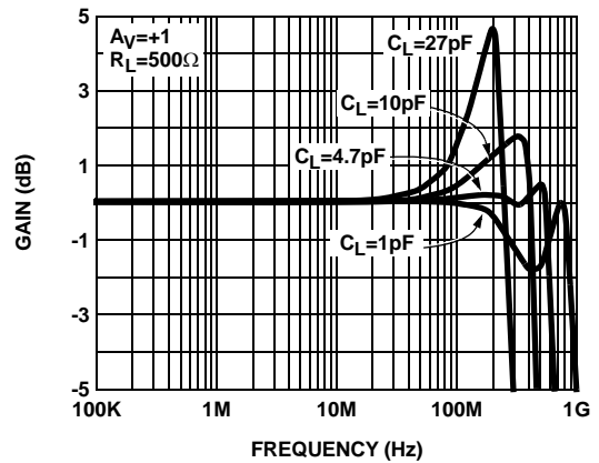
FIGURE 4. SMALL SIGNAL FREQUENCY RESPONSE FOR VARIOUS C_L
