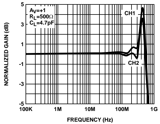
FIGURE 18. CHANNEL TO CHANNEL FREQUENCY RESPONSE
