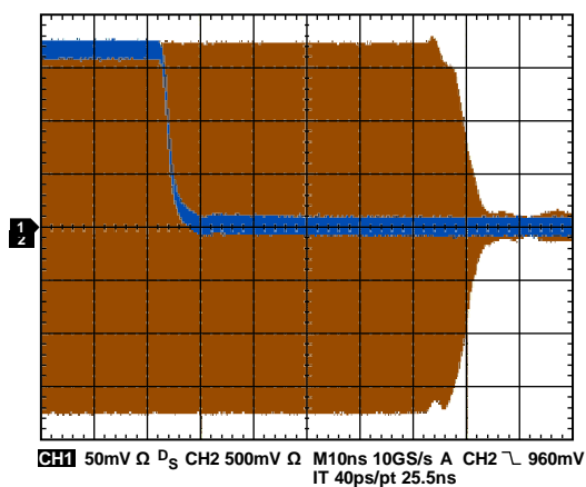
Figure 33. Turn-Off Time, 50% of Control Pulse to 50% of RF Burst
