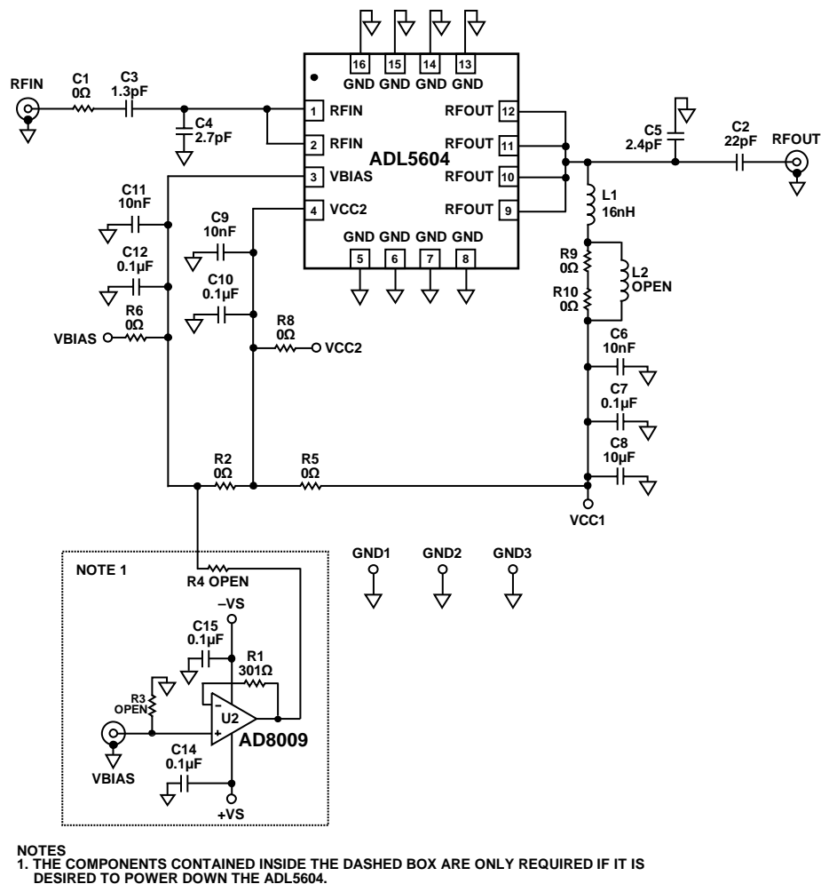
Figure 35. Basic Connections
