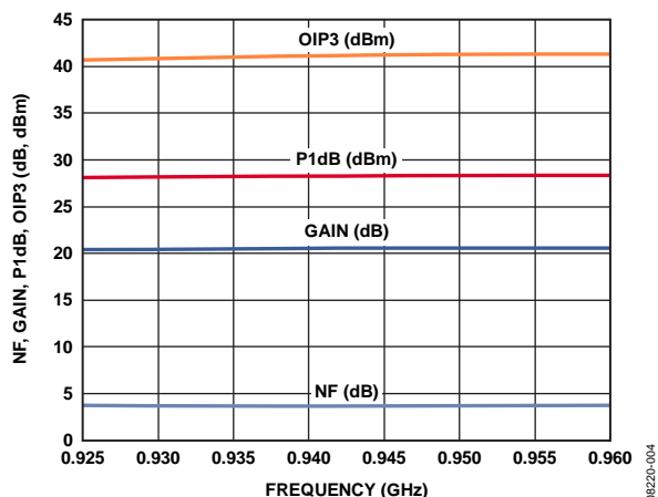
Figure 4. Gain, P1dB, OIP3 at P_{OUT}=14 dBm/Tone and Noise Figure vs. Frequency
