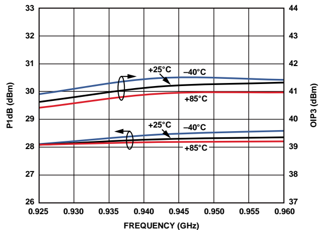
Figure 7. OIP3 at P_{OUT}=14 dBm/Tone and P1dB vs. Frequency and Temperature
