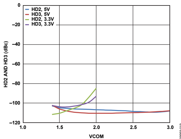
Figure 20. Harmonic Distortion (HD2/HD3) vs. VCOM, A_v = 6 \text{ dB} , V_{POS} = 3.3 \text{ V} and V_{POS} = 5 \text{ V}
