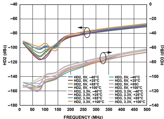
Figure 18. Harmonic Distortion (HD2/HD3) vs. Frequency, Over Temperature, Output Level at 2 V p-p Composite, R_L = 200 \Omega , A_v = 6 \text{ dB} , V_{POS} = 3.3 \text{ V} and V_{POS} = 5 \text{ V} , Four Temperatures
