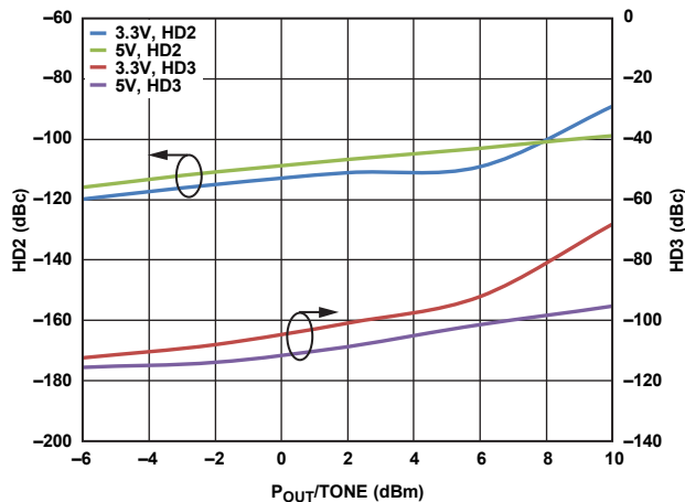
Figure 19. Harmonic Distortion vs. Output Power per Tone, Frequency = 100 MHz, R_L = 200 \Omega , V_{POS} = 3.3 \text{ V} and V_{POS} = 5 \text{ V}
