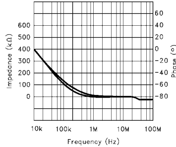
I_{N+} Input Impedance during HOLD, V_S = \pm 5V
