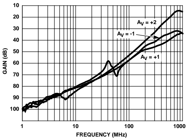
FIGURE 32. REVERSE ISOLATION
