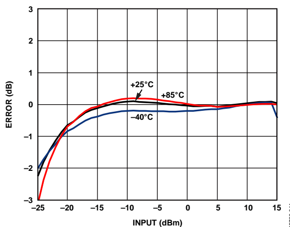
Figure 41. Error from Linear Reference vs. Input at -40^\circ\text{C} , +25^\circ\text{C} , and +85^\circ\text{C} vs. +25^\circ\text{C} Linear Reference, 1900 MHz Frequency, 3.0 V Supply
