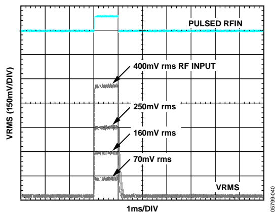
Figure 40. Output Response to Various RF Input Pulse Levels, Supply = 3 V, Frequency = 900 MHz; Square-Domain Filter Open; C_{OUT} = 0.1 \mu\text{F} with Parallel 1 \text{ k}\Omega
