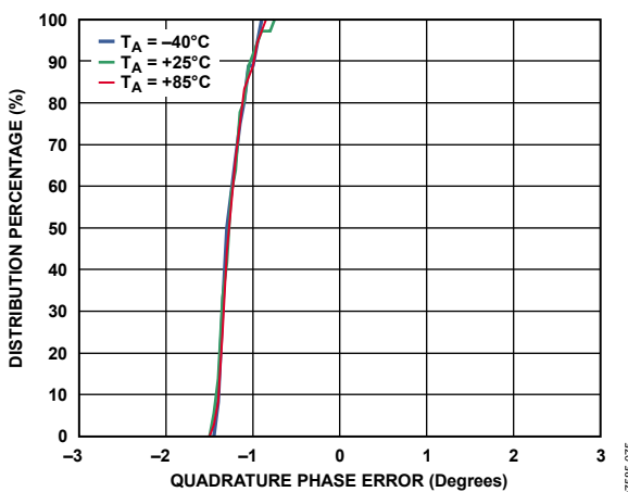
Figure 75. IQ Quadrature Phase Error Distributions
