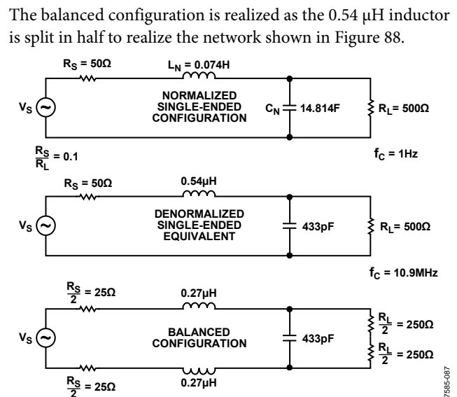
Figure 88. Second-Order Butterworth, Low-Pass Filter Design Example
