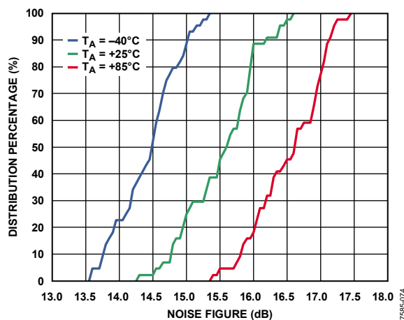
Figure 74. Noise Figure Distributions
