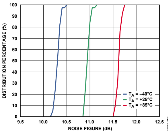
Figure 50. Noise Figure Distributions
