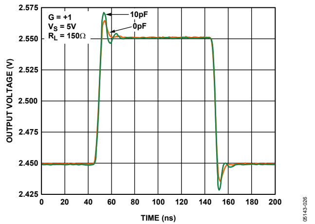
Figure 22. Small Signal Transient Response for Capacitive Load
