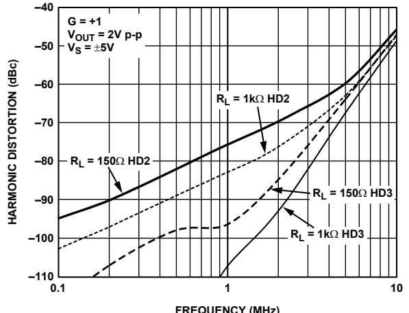
Figure 17. Harmonic Distortion vs. Frequency for Various Loads
