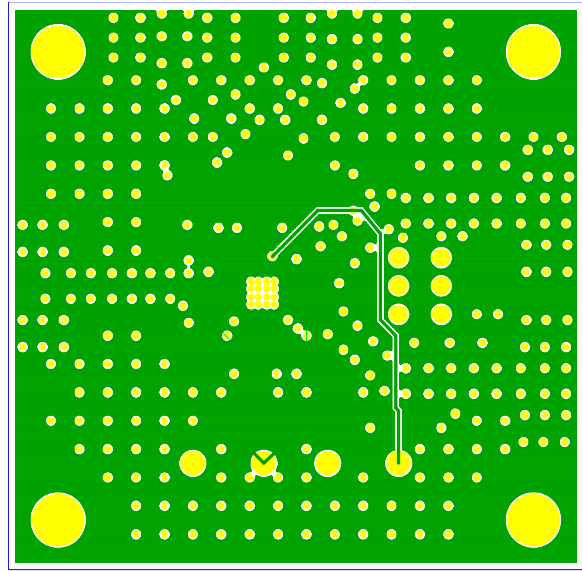
Figure 54. Evaluation Board Power Plane, Internal Layer 2
