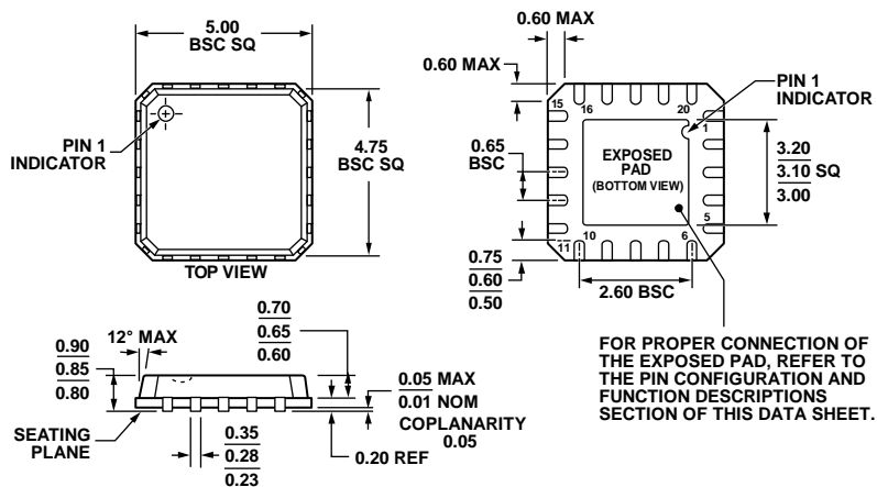
COMPLIANT TO JEDEC STANDARDS MO-220-VHHC Figure 56. 20-Lead Lead Frame Chip Scale Package [LFCSP_VQ] 5 mm × 5 mm Body, Very Thin Quad (CP-20-5) Dimensions shown in millimeters
