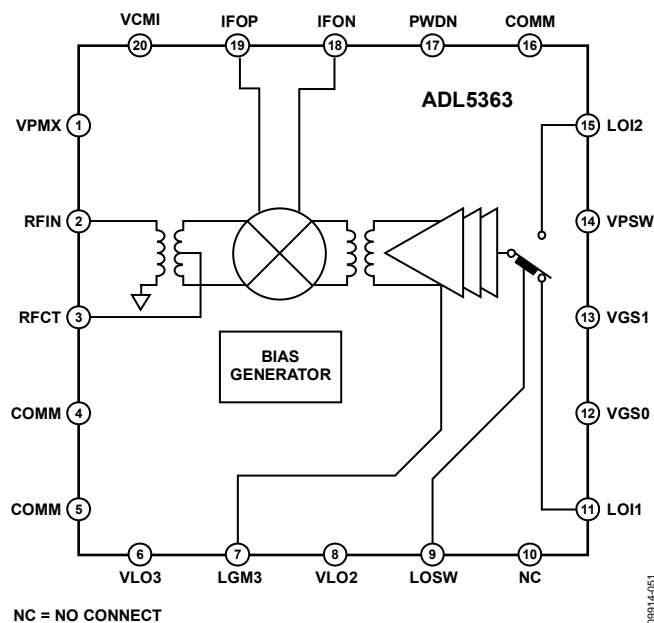
Figure 48. Simplified Schematic
