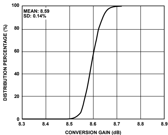
Figure 27. Power Conversion Gain Distribution
