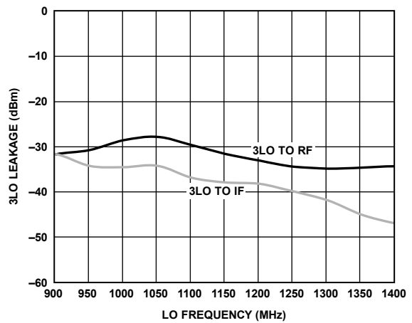
Figure 38. 3LO Leakage vs. LO Frequency
