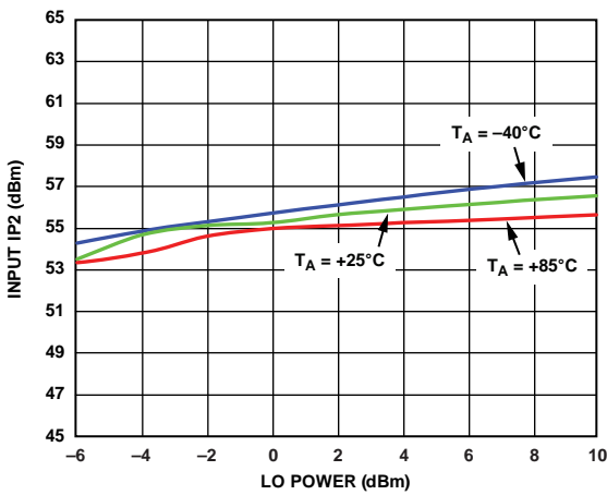
Figure 23. Input IP2 vs. LO Power
