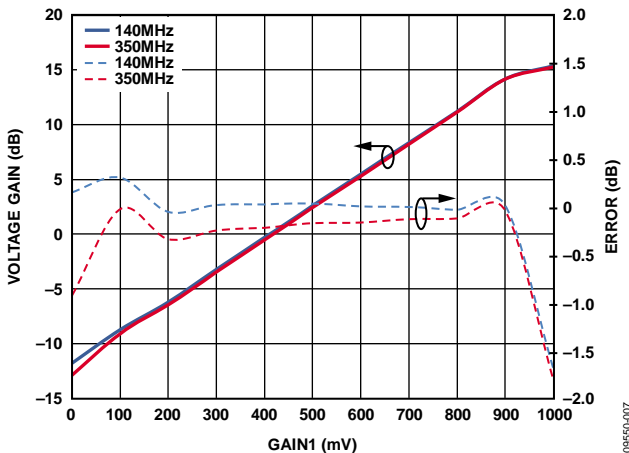
Figure 7. Gain vs. V_{\text{GAIN}} over Frequency at Gain Code 11 for VGA1
