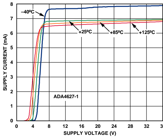
Figure 11. Supply Current vs. Supply Voltage and Temperature
