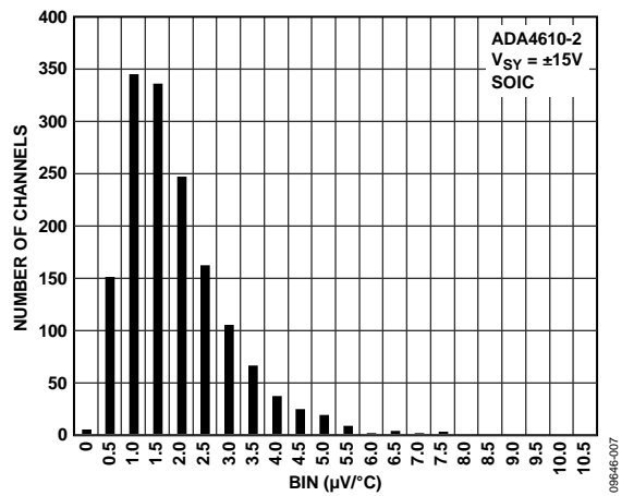
Figure 7. T c V os Distribution
