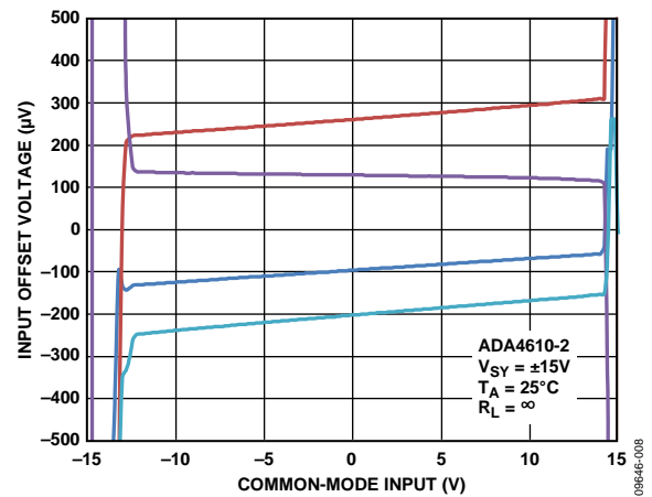
Figure 8. Input Offset Voltage vs. Common-Mode Input Voltage
