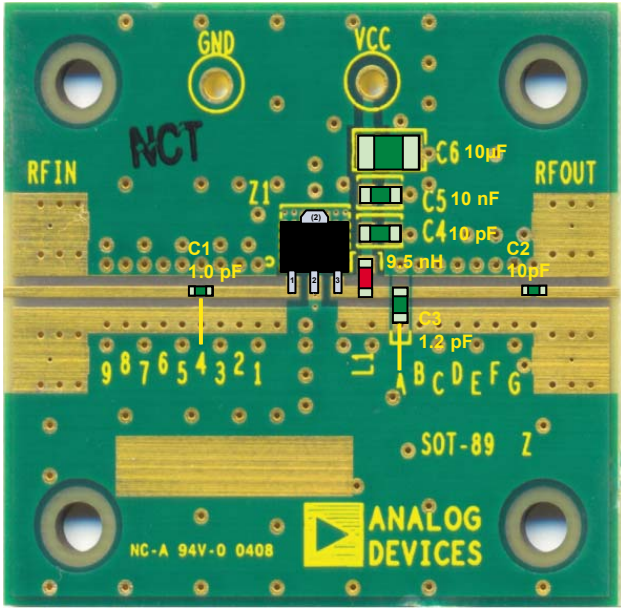
Figure 28. Evaluation Board Layout and Default Component Placement for Operation from 2500 MHz to 2700 MHz (Note: C7 Is Not Placed)
