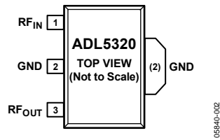
Figure 2. Pin Configuration
