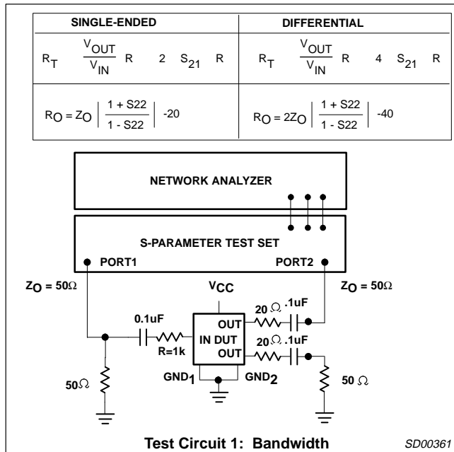
Figure 2. Test Circuit1
