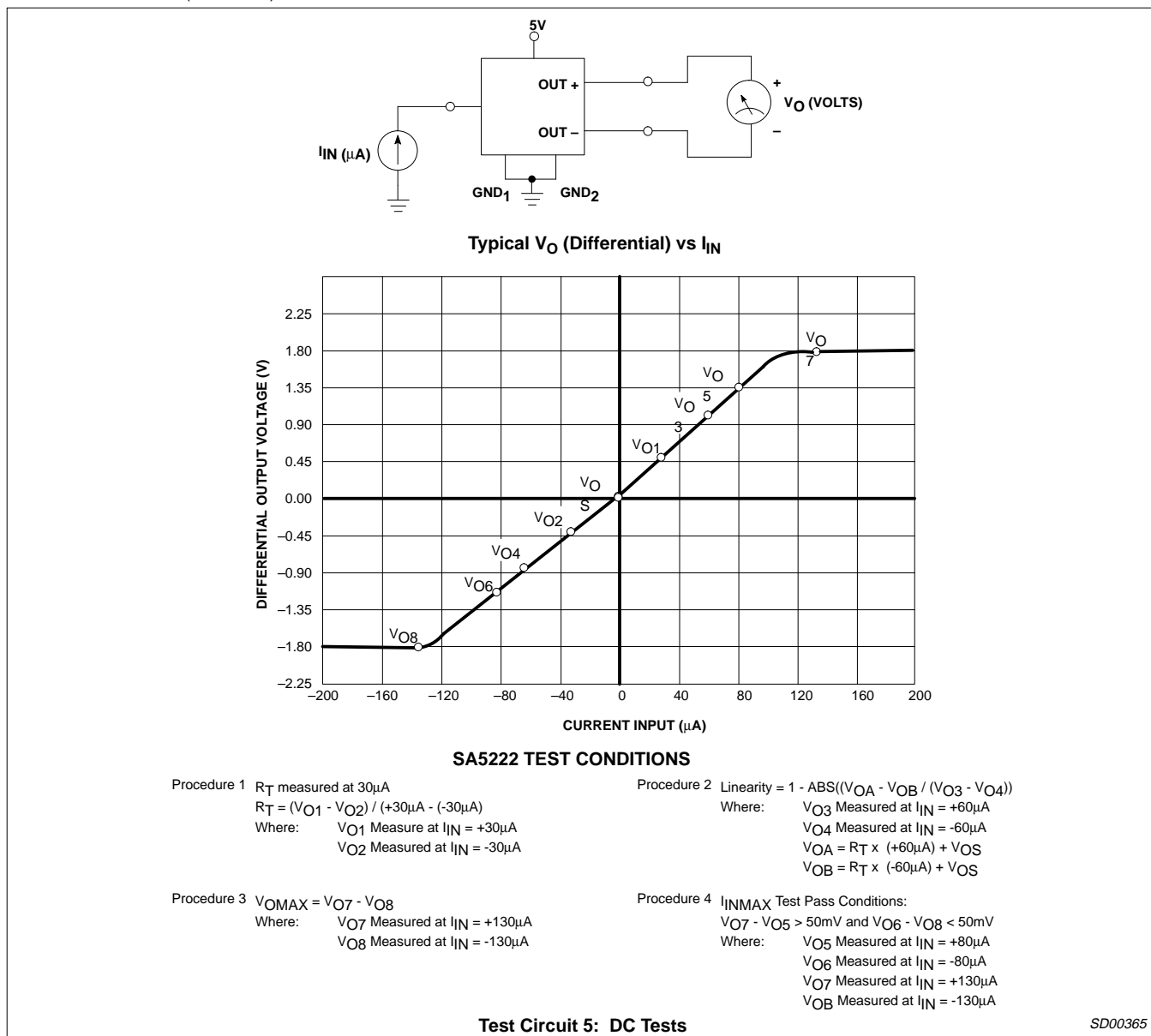
Figure 6. Test Circuit5
