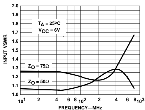
Figure 11. Input VSWR vs Frequency
