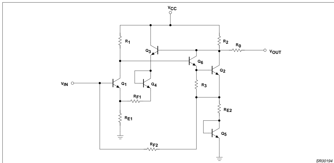
Figure 2. Equivalent Schematic
