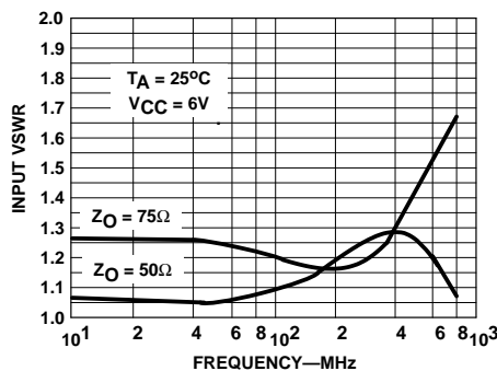
a. Input VSWR vs Frequency
