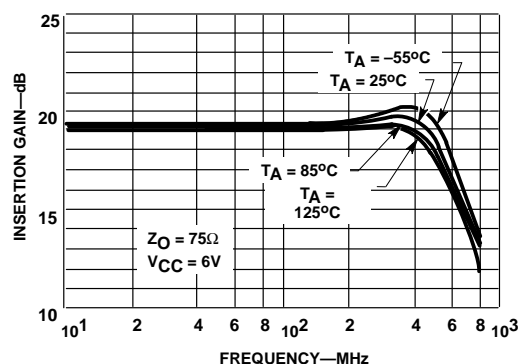
Figure 16. Insertion Gain vs Frequency ( S_{21} )
