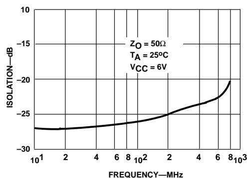
Figure 14. Isolation vs Frequency ( S_{12} )
