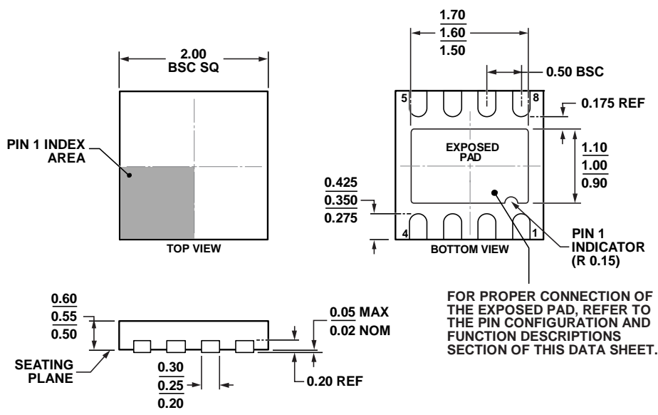
Figure 50. 8-Lead Lead Frame Chip Scale Package [LFCSP_UD]
