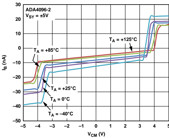
Figure 17. Input Bias Current vs. V_{CM} and Temperature
