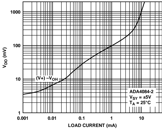
Figure 32. Dropout Voltage vs. Source Current
