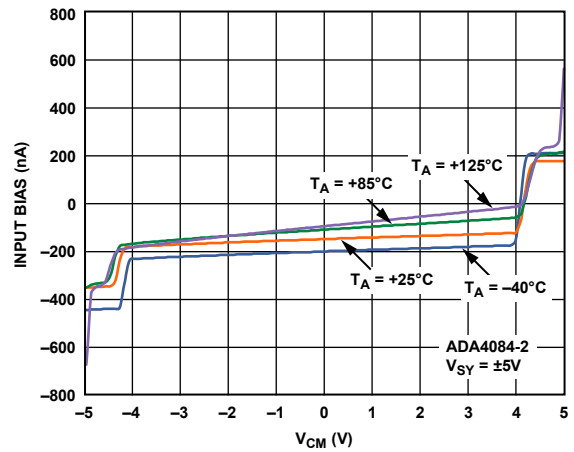
Figure 31. Input Bias Current vs. VCM and Temperature
