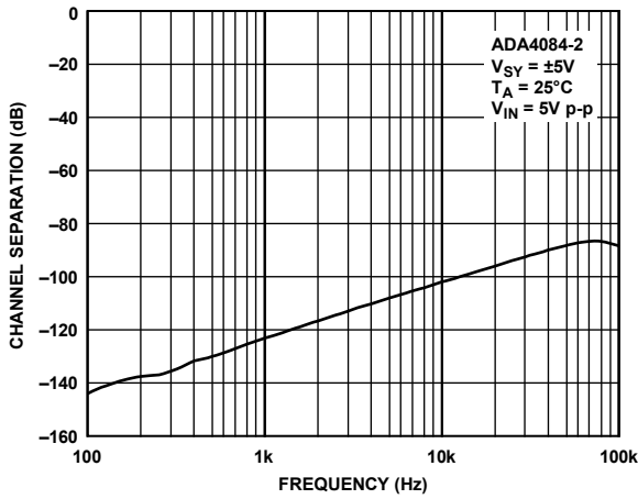
Figure 45. Channel Separation
