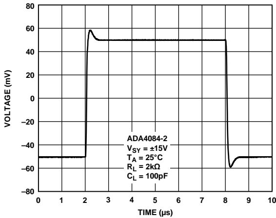
Figure 63. Small Signal Transient Response
