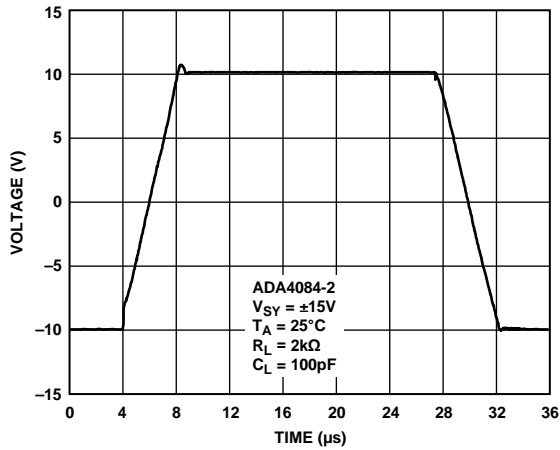
Figure 62. Large Signal Transient Response
