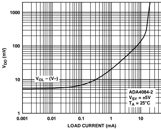
Figure 33. Dropout Voltage vs. Sink Current
