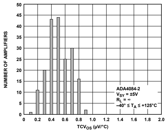
Figure 28. TCVOS Distribution
