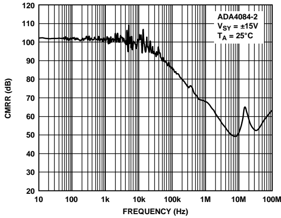
Figure 61. CMRR vs. Frequency
