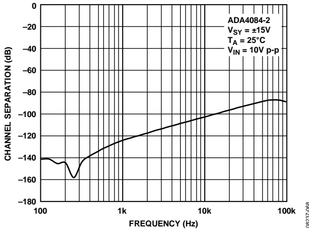
Figure 68. Channel Separation
